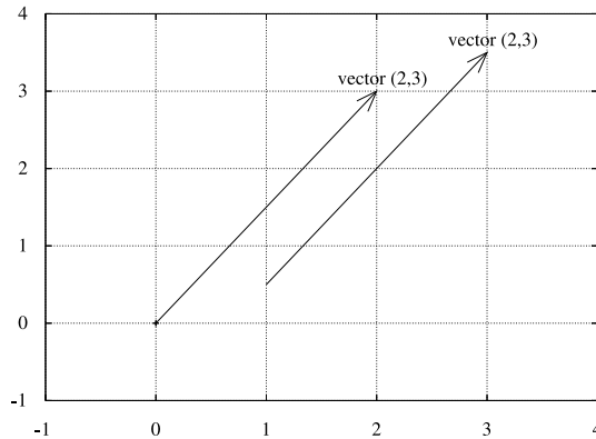
Fig. 5.1 A vector (2,3) visualized in the standard way as an arrow from the origin to the point (2,3) , and mathematically equivalently, as an arrow from (1, \frac{1}{2}) (or any point (a,b) ) to (3, 3\frac{1}{2}) (or (a+2, b+3) ).
