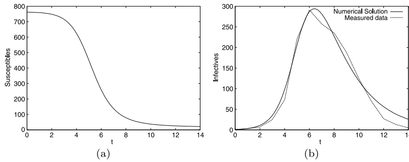
Fig. C.4 Graphs of (a) susceptibles and (b) infectives for an influenza in a British boarding school in 1978.
